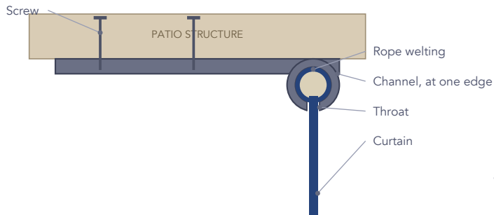
HEAD — rope welting captured in the track
