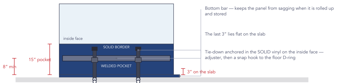
SILL — the panel sits ON the ground (inside face shown)
